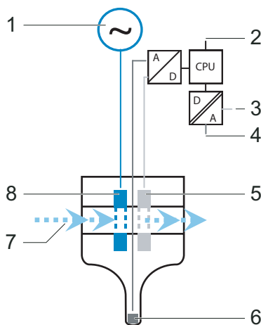
Fig. 2. Measuring principle
