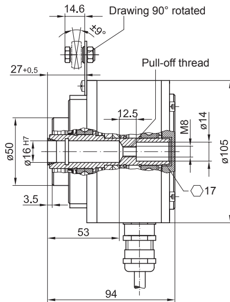
Blind hollow shaft
