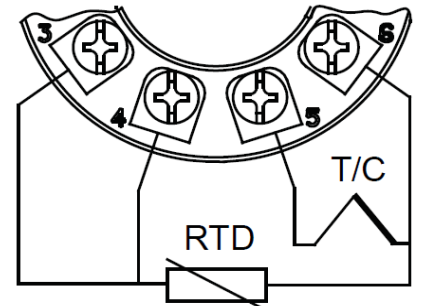
External CJC-compensation, 3-wire cable compensation
