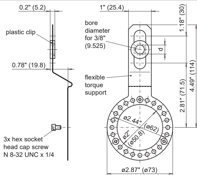
Butoir anti-rotation T5
