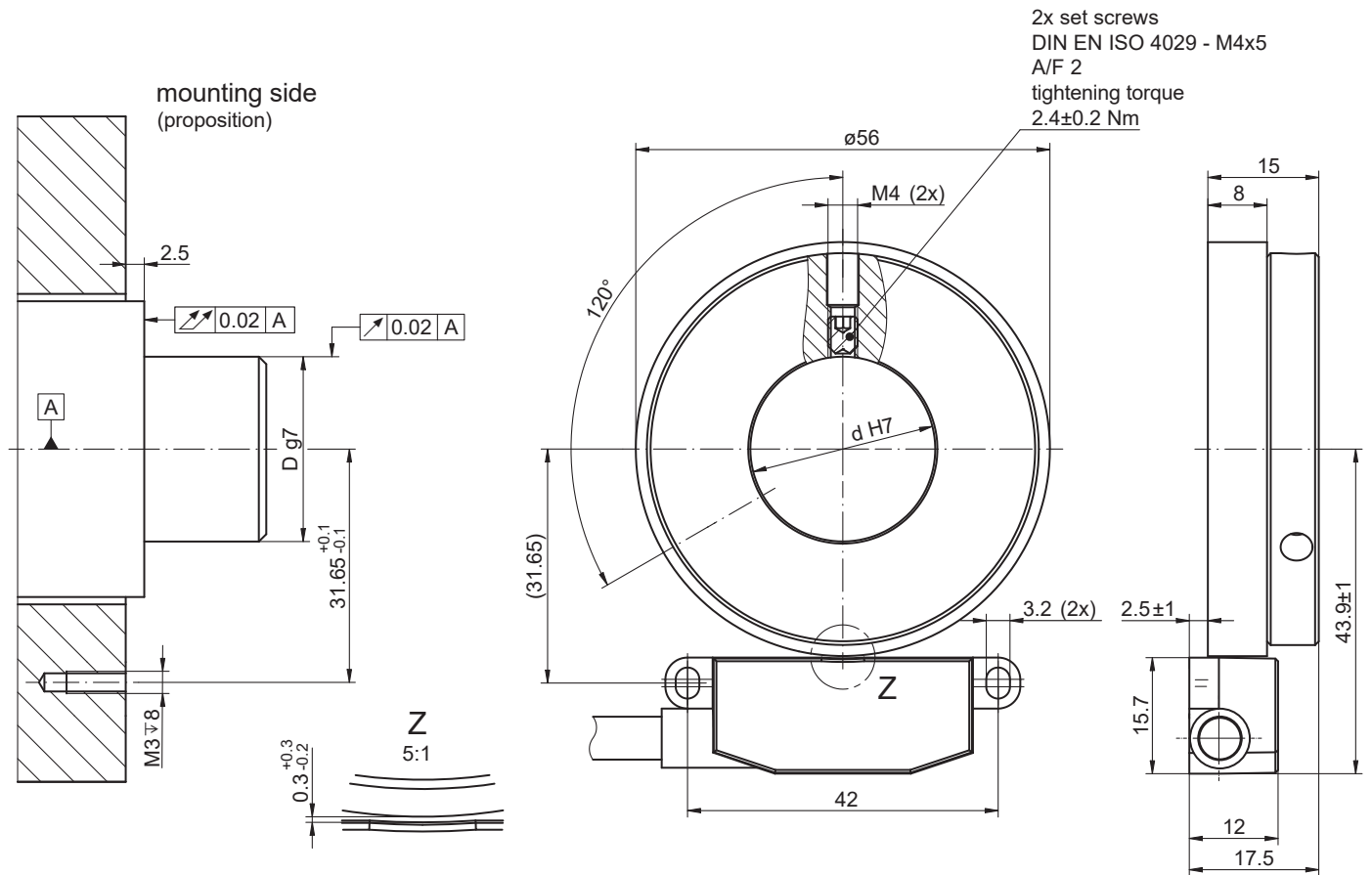
EB200E.IR-FN with EBS.R-FN064.S for screw mounting
