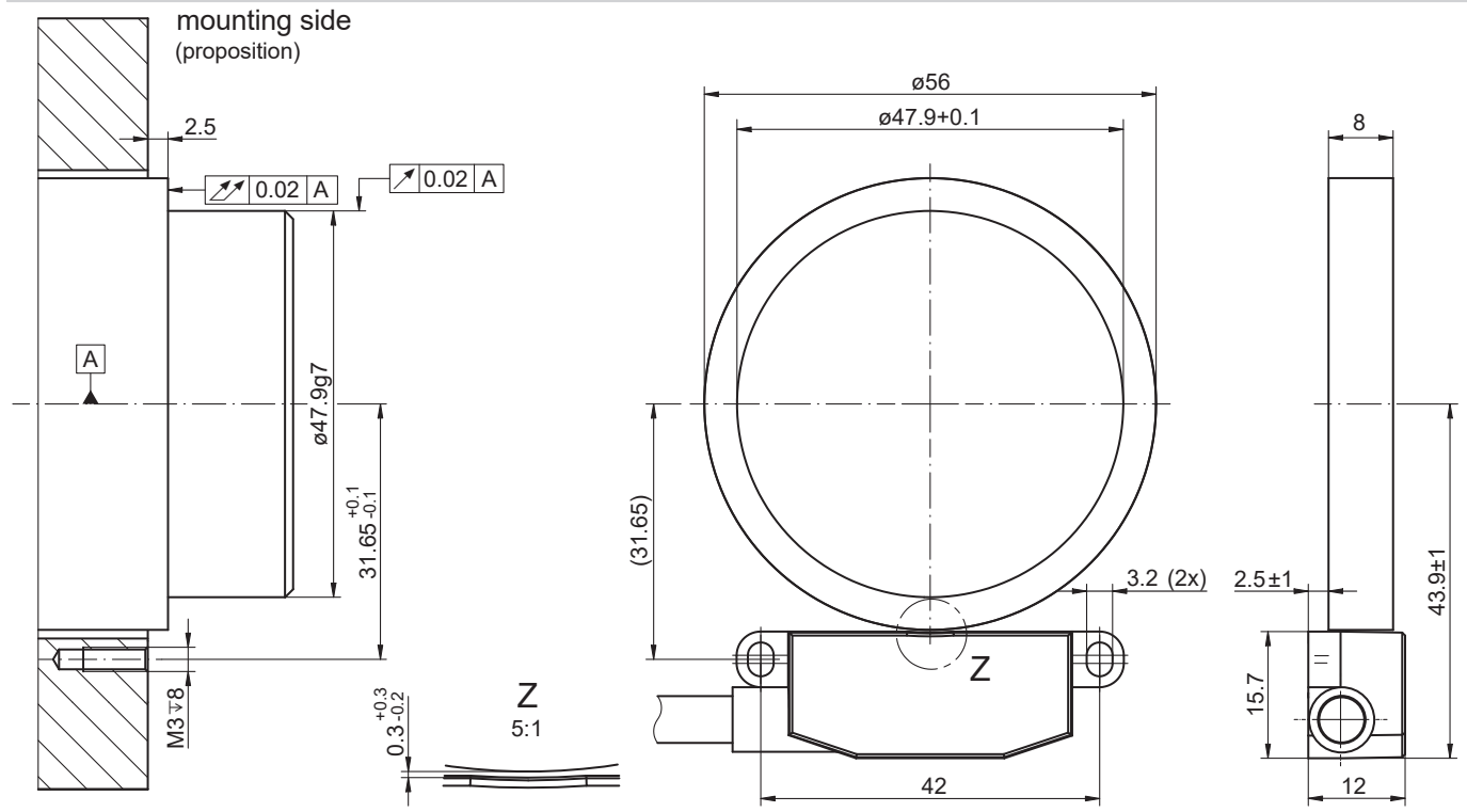
EB200E.IR-FN with EBS.R-FN064.B for bonding
