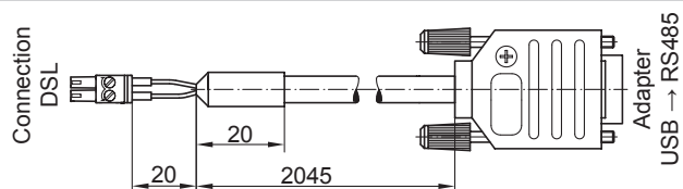
Connecting cable for DSL-RS485 interface
