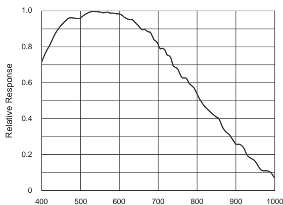
Sony® IMX 545 mono Wave Length [nm]
