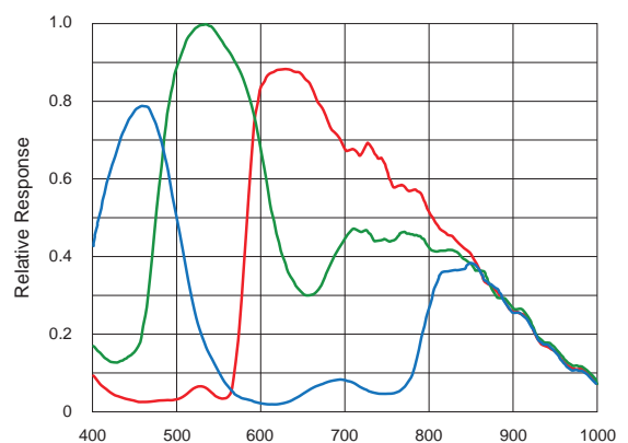
Sony® IMX 545 color Wave Length [nm]
