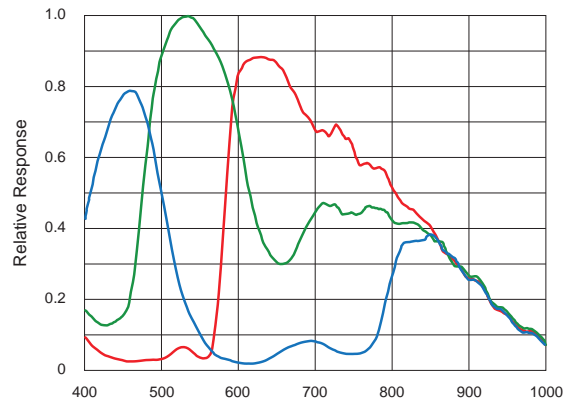
Sony® IMX 546 color Wave Length [nm]
