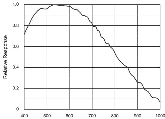
Sony® IMX 546 mono Wave Length [nm]
