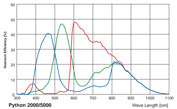
Python 2000/5000 Wave Length [nm]
