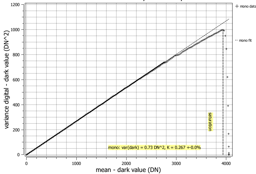
Photon transfer mACC300218, 533 nm, 27.07.2023
