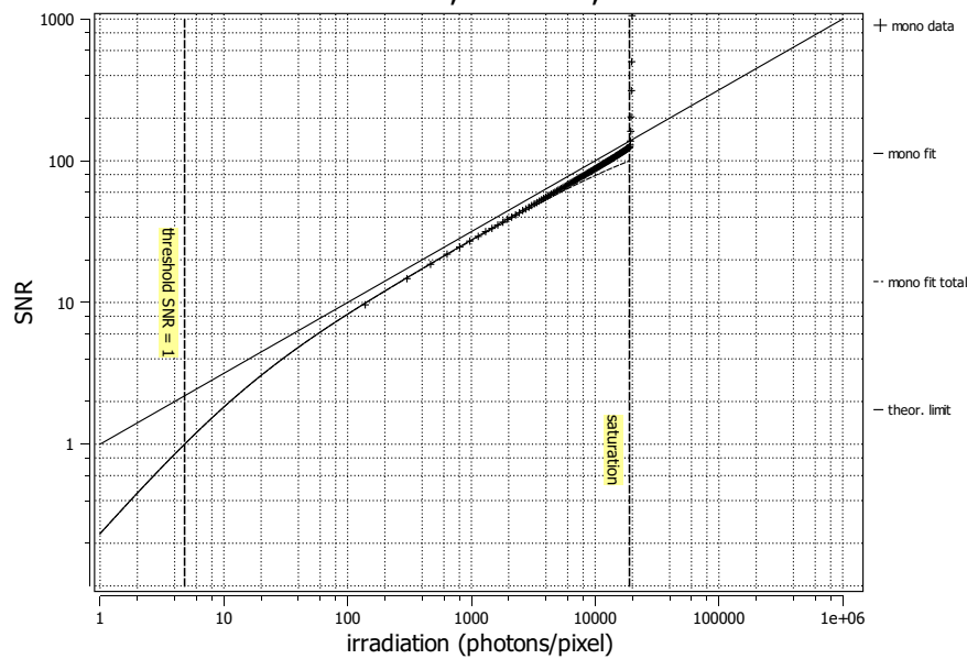
SNR mACC300218, 533 nm, 27.07.2023
