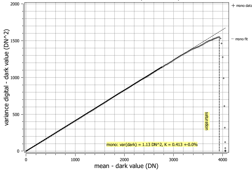
Photon transfer mACC300212, 533 nm, 26.07.2023
