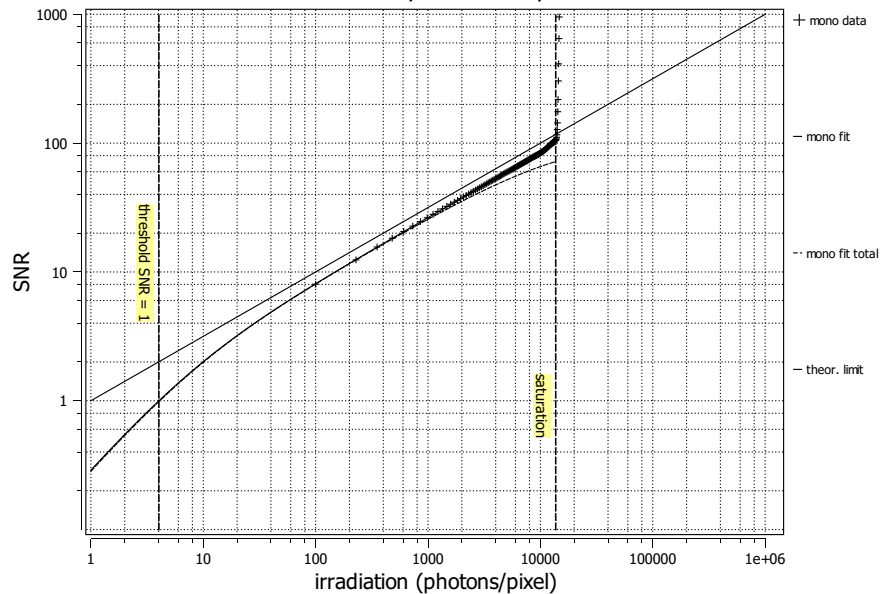
SNR mACC300200, 533 nm, 17.07.2023
