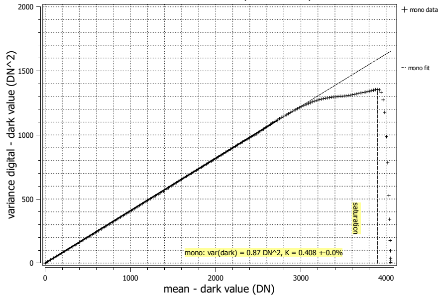
Photon transfer mACC300200, 533 nm, 17.07.2023
