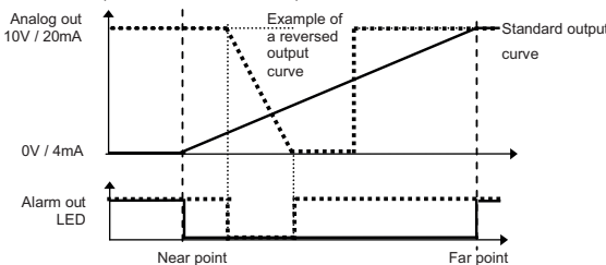
Example of a reverse taught measuring range: 4 mA / 0 V in the far point, 20 mA / 10 V in the near point
